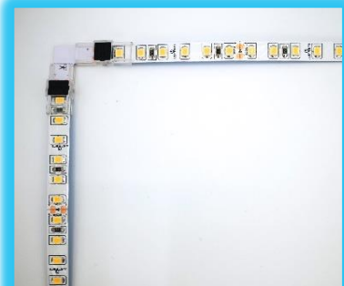
2 - Slide LED strip & L-Strip Connector into each end of Beetle Clip & compress firmly with pliers
