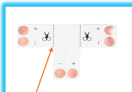
1 - Trim T-Strip Connector where scissors are pictured to convert it to an L-Strip Connector
